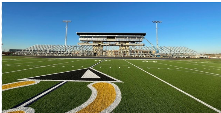
Site: Stadium bleacher framing installation in progress.
